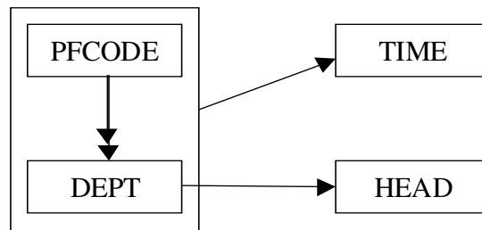
Dependency Diagram
